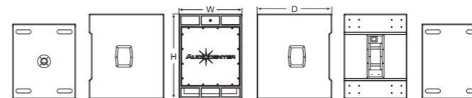
Dimension(W×H×D): 520×700×618mm
