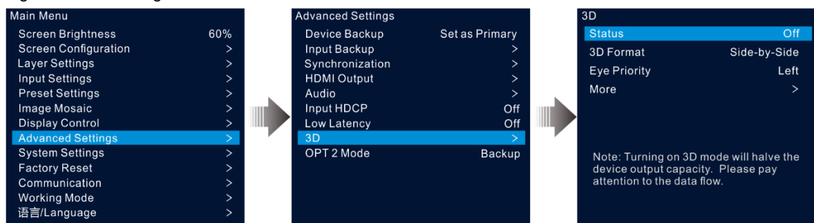
Figure 5-39 3D settings
