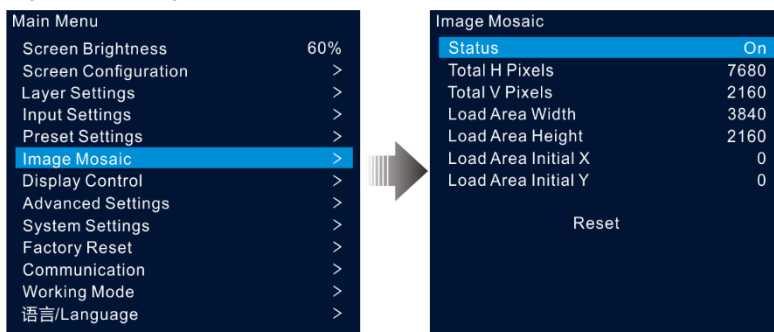
Figure 5-23 Image mosaic
